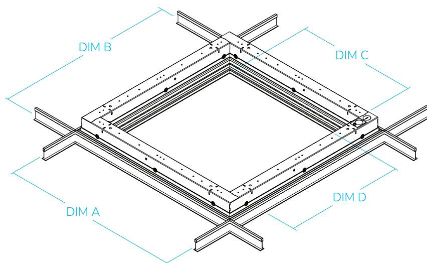
On-Center Grid Dimensions
