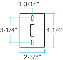
Mounting Plate Dimensions
