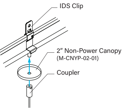
Grid Mounting
