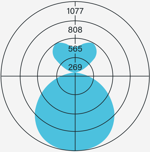
L6DI-A-70-840 70% Direct, 30% Indirect Lumens/ft 600 Lumens/watt 103
