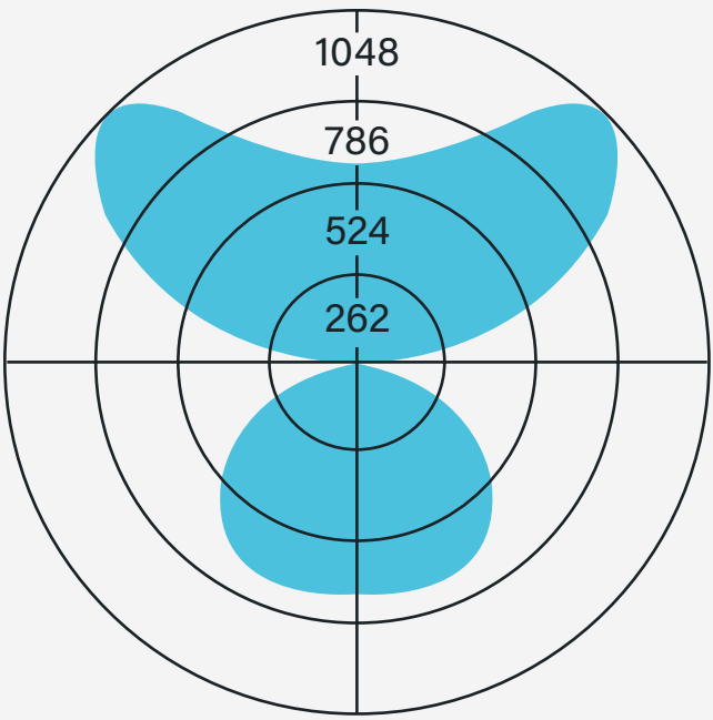
L6DI-A-40-840HO 40% Direct, 60% Indirect Lumens/ft 850 Lumens/watt 151.7
