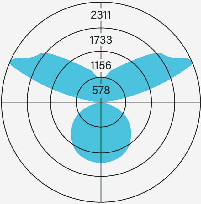
L6DI-A-BW-840VHO-840VHO Dual Output, Batwing Indirect Lumens/ft Direct - 1250, Indirect - 1250 Lumens/watt 99.6
