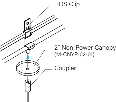
Grid Mounting
