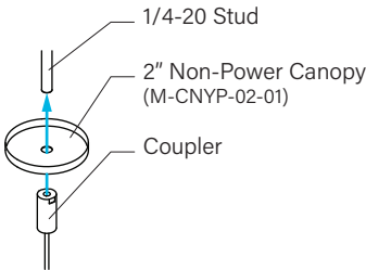
Inaccessible Mounting
