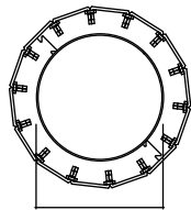
Finadrum Light Engine 21-15/16" (557.7mm)
