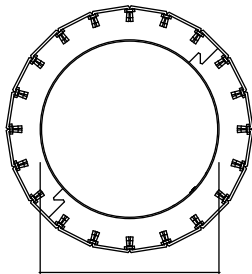
Finadrum Light Engine 33-15/16" (862.5mm)
