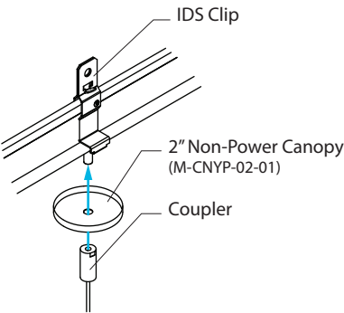
Grid Mounting
