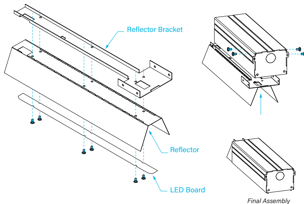
Final Assembly
