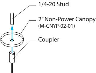
Inaccessible Mounting
