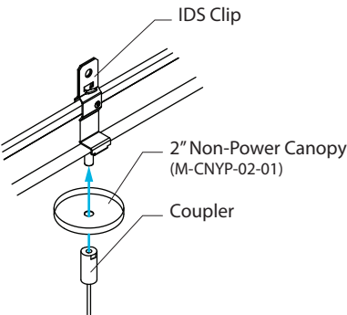
Grid Mounting
