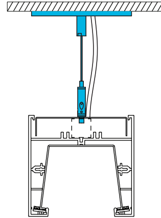
AC - Single, Adjustable AC Cable
