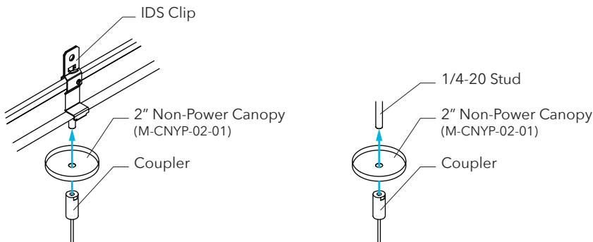
Grid Mounting
