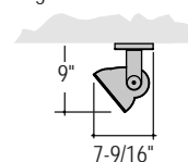
Ceiling Mount
