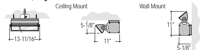
DF - Decorative Flush, Integral Ballast
