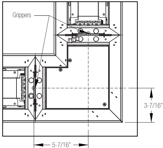
Linero 6 Curved L Corner
