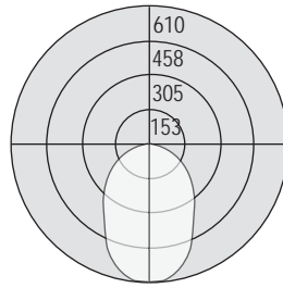
Test # 203131 Part #: EX4-R-N-1T8 Total Efficiency: 46%
