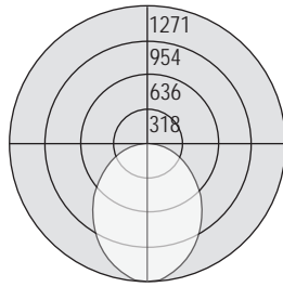
Test # 203132 Part #: EX4-R-N-2T5 Total Efficiency: 54.8%
