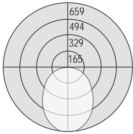
Test # 203129 Part #: EX4-R-N-1T5 Total Efficiency: 56.9%
